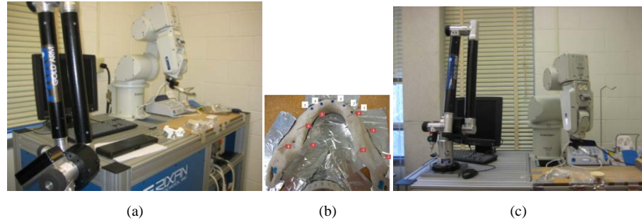
Figure 4 (a) Previous phantom experiments setup; (b) Fiducials ( italic letters ) and registration points ( normal letters ); (c) Modified phantom experiments setup
