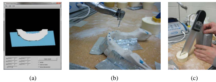
Figure 5 3D model on the reference plane in (a) the virtual and (b) the reference/ operation CS
